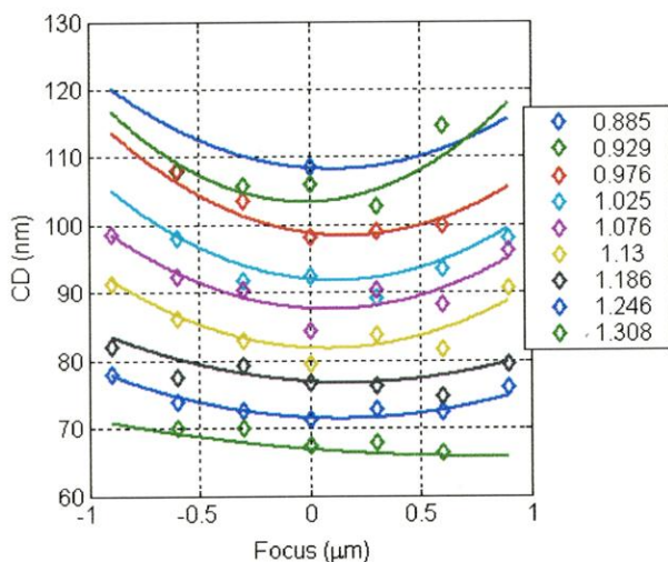
Fig. 6. +/-10% CD change process-window results for 90-nm half-pitch features.
