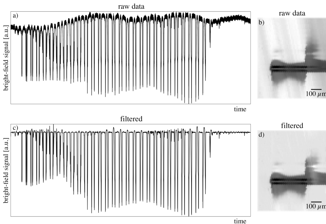
Fig. 2. Large area scans of a region showing high-powered UV laser damage, raw and filtered -data reconstructions. Without filtering ( a , b ), fluctuations in the illumination flux level can appear as large-scale changes in the apparent reflectivity that follow the direction of the scanning path, slightly inclined from vertical. Intensity-level filtering ( c , d ) is most effective in regions surrounded by open mask areas. In this example, the largest reflectivity change occurs in the dark regions, where the reflectivity falls to 31% of the background level.
