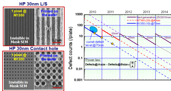
(a) Inspection tool : Minimum size of defect (b) Blank quality : Total number of defect
