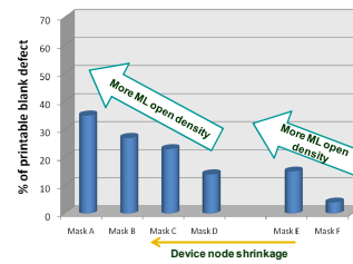
Figure 17. Printability of blank defect
