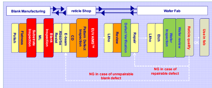
Figure 15. Defect verification process without EUV AIMS™
