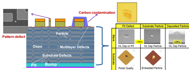
Figure 1. Types of defects on an EUV blank
