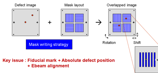
Figure 20. Fiducial mark for defect mitigation technology
