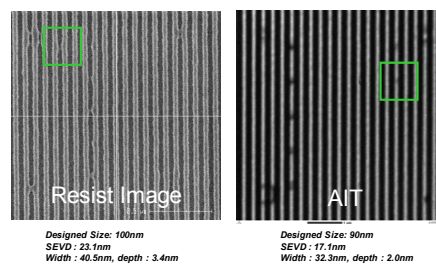
Figure 5. Minimum printable pit defect on 35nm HP
