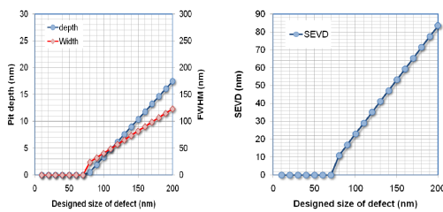
Figure 3. Size and depth of programmed pit defect
