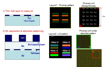
Figure 4. Reticle description with programmed pit defect
