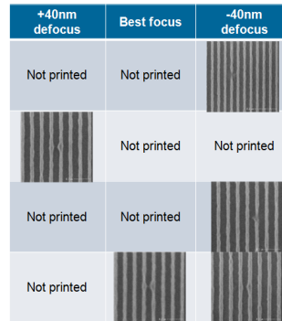
Figure 8. Focus dependency of blank defects
