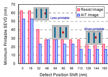
Figure 5. Minimum printable pit defect on 35nm HP
