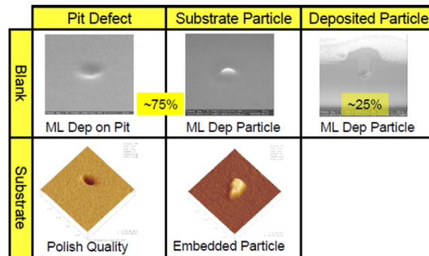
Figure 1. Types of defects on an EUV blank
