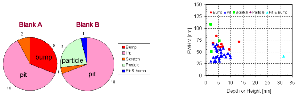
Figure 5. Pareto chart of defects in 2 test blanks Figure 6. Defect profile of each defect using the AFM
