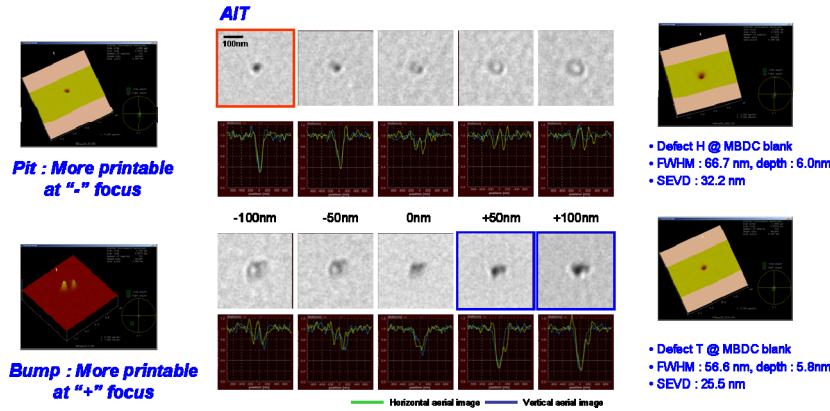
Figure 9. Printability as through-focus of bumps and pits
