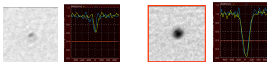
(a) Unprintable blank defect
