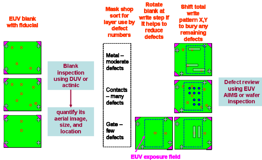
Figure 12. Strategy of defect mitigation for EUV masks
