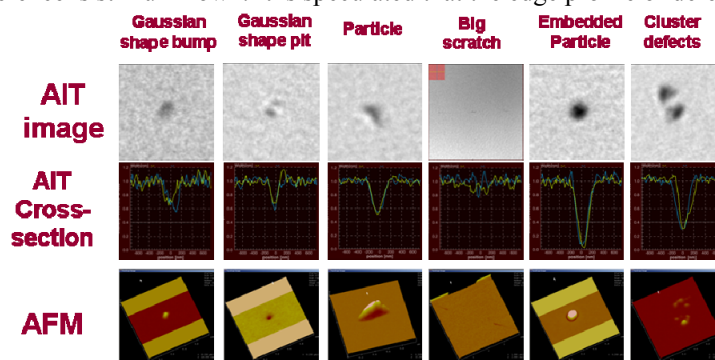
Figure 8. Examples of real defects from the AIT and AFM
