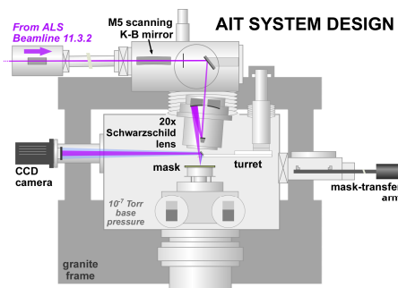
Figure 4. AIT system design
