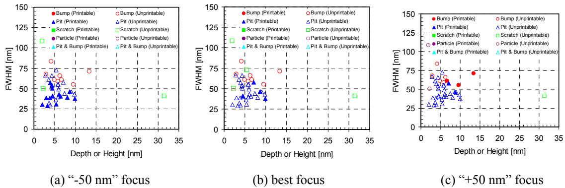
Figure 11. Defect printability as through-focus
