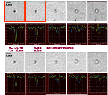
Figure 10. Printability of defects of similar sizes and pit defects
