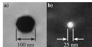
FIG 3. Free-standing Ni-membrane pinholes used to create spherical reference waves. (a) SEM micrograph of an object-side pinhole. (b) TEM micrograph of an image-side pinhole.
