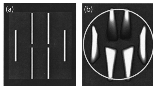
FIG. 3. (a) Modeled pupil fill for the central field point. (b) Open frame pupil illumination, measured on a scintillator at the pupil of the POB. The circle denotes \sigma=0.7 .
