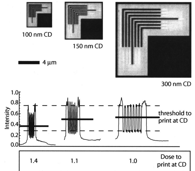
FIG. 10. Modeled aerial images of elbow patterns of various sizes showing that, for these particular mask patterns, flare increases with increasing feature size.
