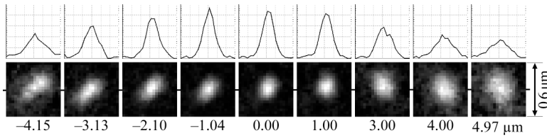
Fig. 14. Images of one 175-nm (35-nm) contact, followed through focus, reveal a sharp point-spread function, yet several microns of astigmatic displacement. Each image and profile are 600-nm wide. Relative focus displacements are given below each image, in \mu\text{m} . The images are centered on the points of maximum intensity, and horizontal line profiles through those points are shown.
