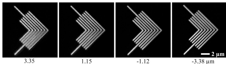
Fig. 12 (above). 45° astigmatism is visible in this series of images of 250-nm (50-nm) dark-field elbows. The same contrast analysis through focus used in the CTF calculations is here used to identify the best focus planes for the two directions. The relative z position of each image is shown in \mu\text{m} .
