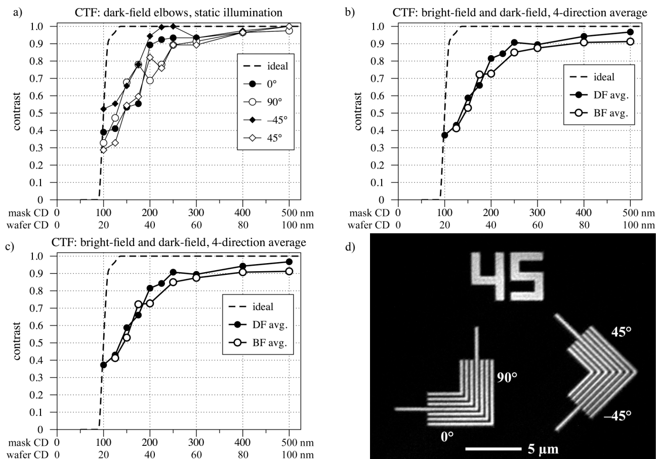
Fig. 10. Calculation of the CTF was performed by evaluating contrast in both bright and dark field elbow patterns in four line orientations. (d) A detail of a typical image from a through-focus series, close to focus; the "45" label indicates a 5 \times , wafer equivalent size. The angle definitions assigned to the four branches are shown. (a) CTF calculated for dark-field elbows in all four line-directions. (b) A similar calculation for bright-field scanning illumination. (c) The average contrast values in the two series are compared.
