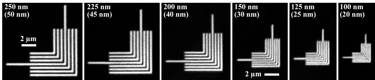
Fig. 9. Representative 0^\circ - 90^\circ elbow patterns used in the calculation of the dark-field CTF. A finite astigmatism magnitude makes the contrast higher in one direction or the other, through focus. These images are close to best focus in each case. All images are shown on the same size scale.
