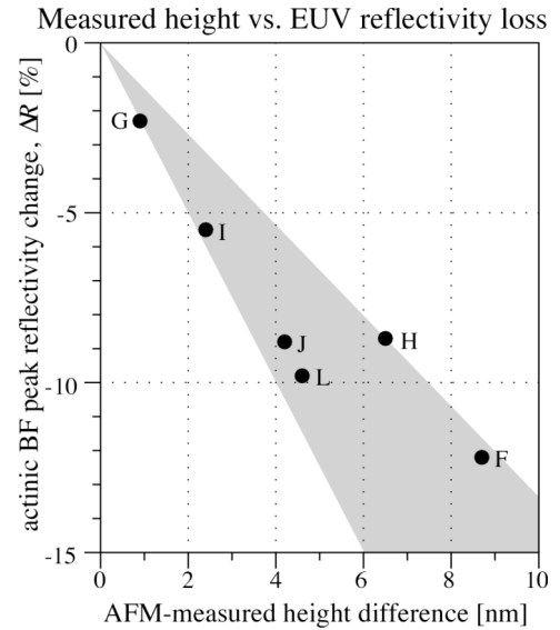
Fig. 4. Observed changes in EUV reflectivity vs. measured AFM height change at surface. There is a broad trend of lowered EUV reflectivity with the additional \text{SiO}_2 thickness.
