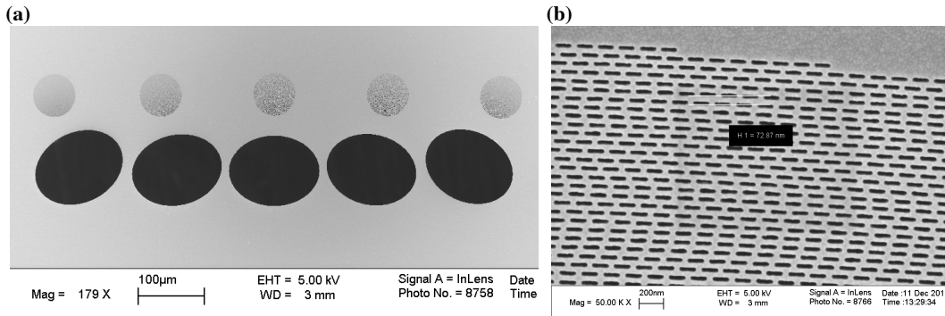
Figure 6. (a) SEM micrograph of a region of the zoneplate array containing five zoneplates and their associated windows. (b) The outer edge of one freestanding zoneplate, showing the stencil structure that gives it strength.
