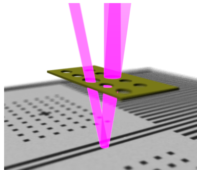
Figure 4. Cartoon of the reflective zoneplate geometry. The incident beam passes through an open window in the absorber membrane and illuminates the mask. The off-axis zoneplate projects the image directly upward to the CCD, while the undiffracted zeroth-order light propagates at a different angle.
