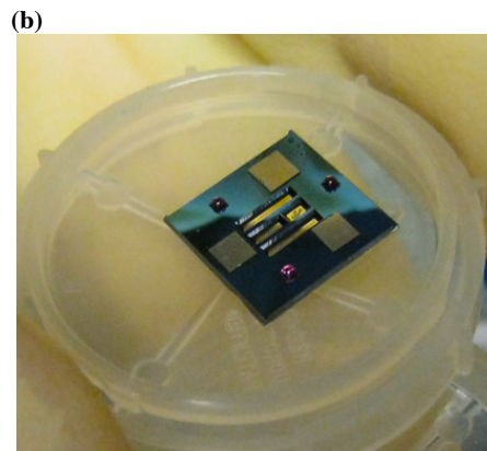
Figure 5. (a) a single zoneplate-array chip mounted onto a removable zoneplate holder. Both the chips and the holder rely on kinematic mounts for accurate, repeatable positioning. (b) The zoneplate array chip is 11-mm wide and contains four free-standing membranes.
